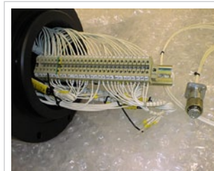
Pressure Housing and Junction Box
